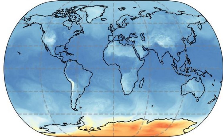
absHumidity (g/m 3 ) @ ground level, summer, 01.07.2020
