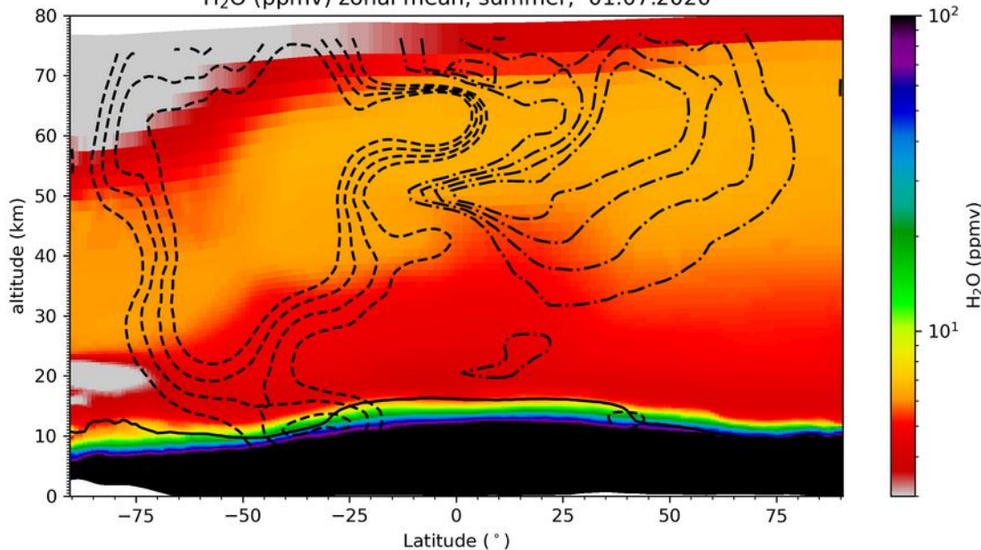
H 2 O (ppmv) zonal mean, summer, 01.07.2020
