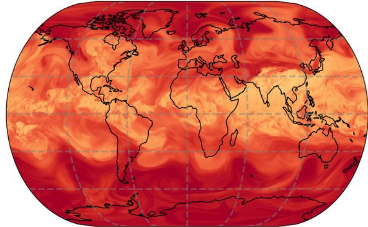
absHumidity (g/m 3 ) @ 200hPa level, summer, 01.07.2020
