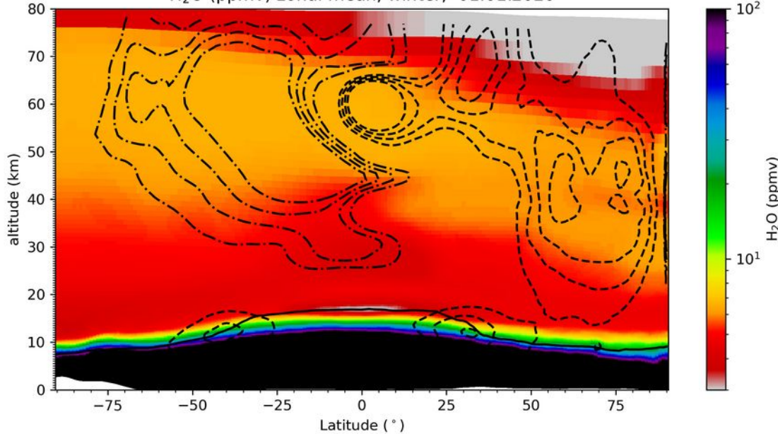
H 2 O (ppmv) zonal mean, winter, 01.01.2020
