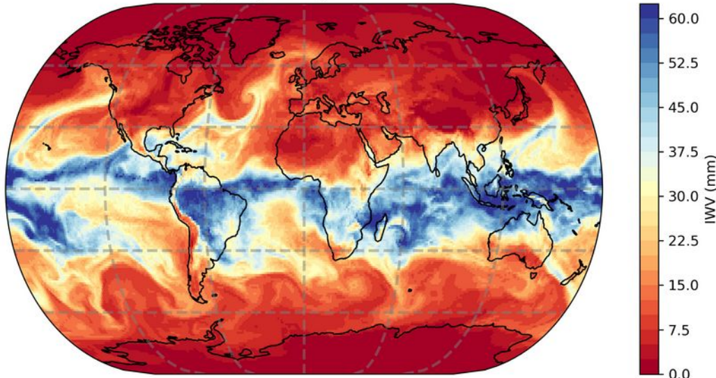
IWV (mm) winter, 01.01.2020
