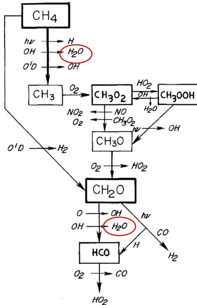
Figure 3. Diagram of the methane oxidation chain of photochemical reactions.
