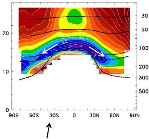
HALOE water vapor March
