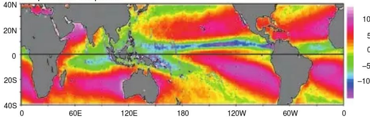
Evaporation-Precipitation
