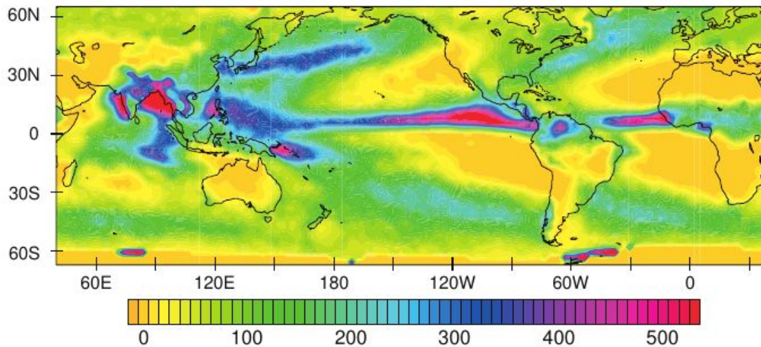
Evaporation-Precipitation
